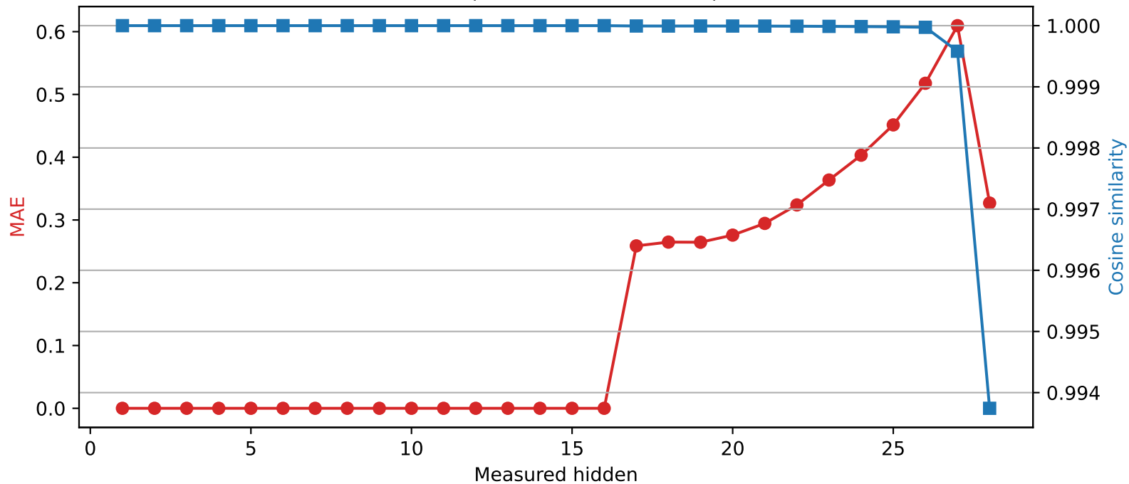
Qwen2.5-7B-Instruct | Quantized layer 16 | float16 → int4
