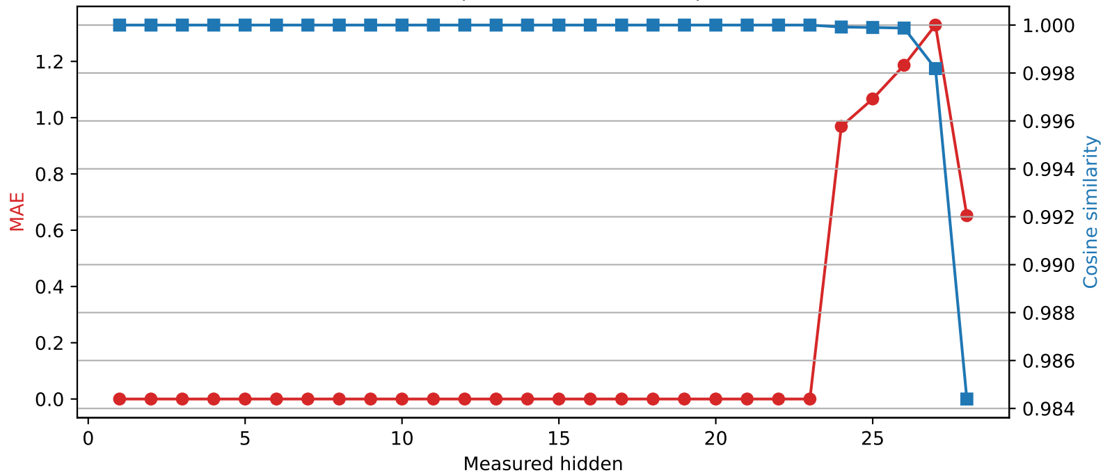
Qwen2.5-7B-Instruct | Quantized layer 23 | float16 → int4
