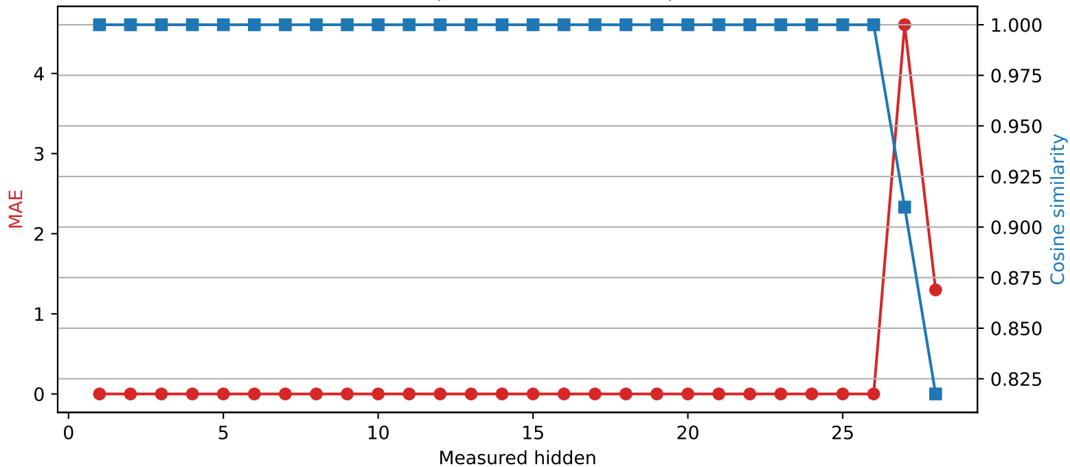
Qwen2.5-7B-Instruct | Quantized layer 26 | float16 → int4
