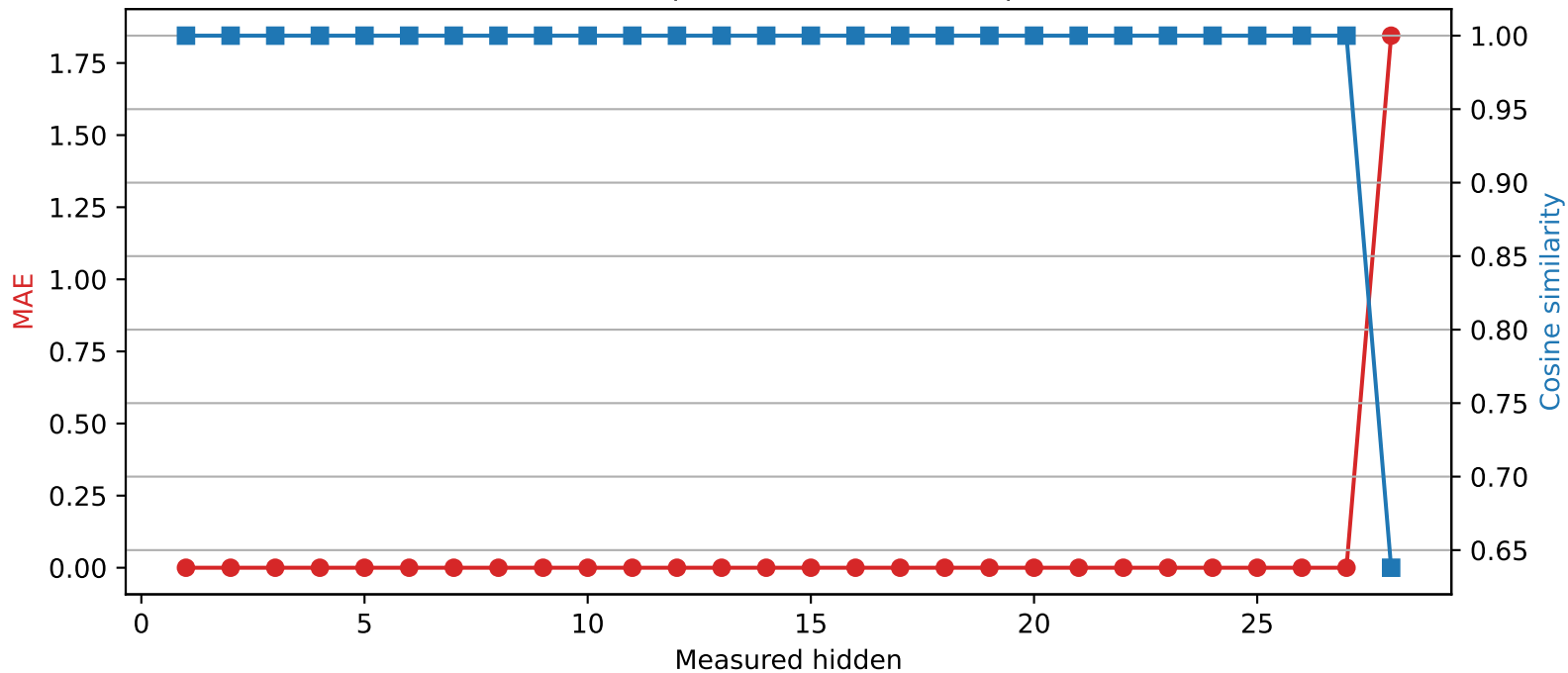
Qwen2.5-7B-Instruct | Quantized layer 27 | float16 \rightarrow int4
