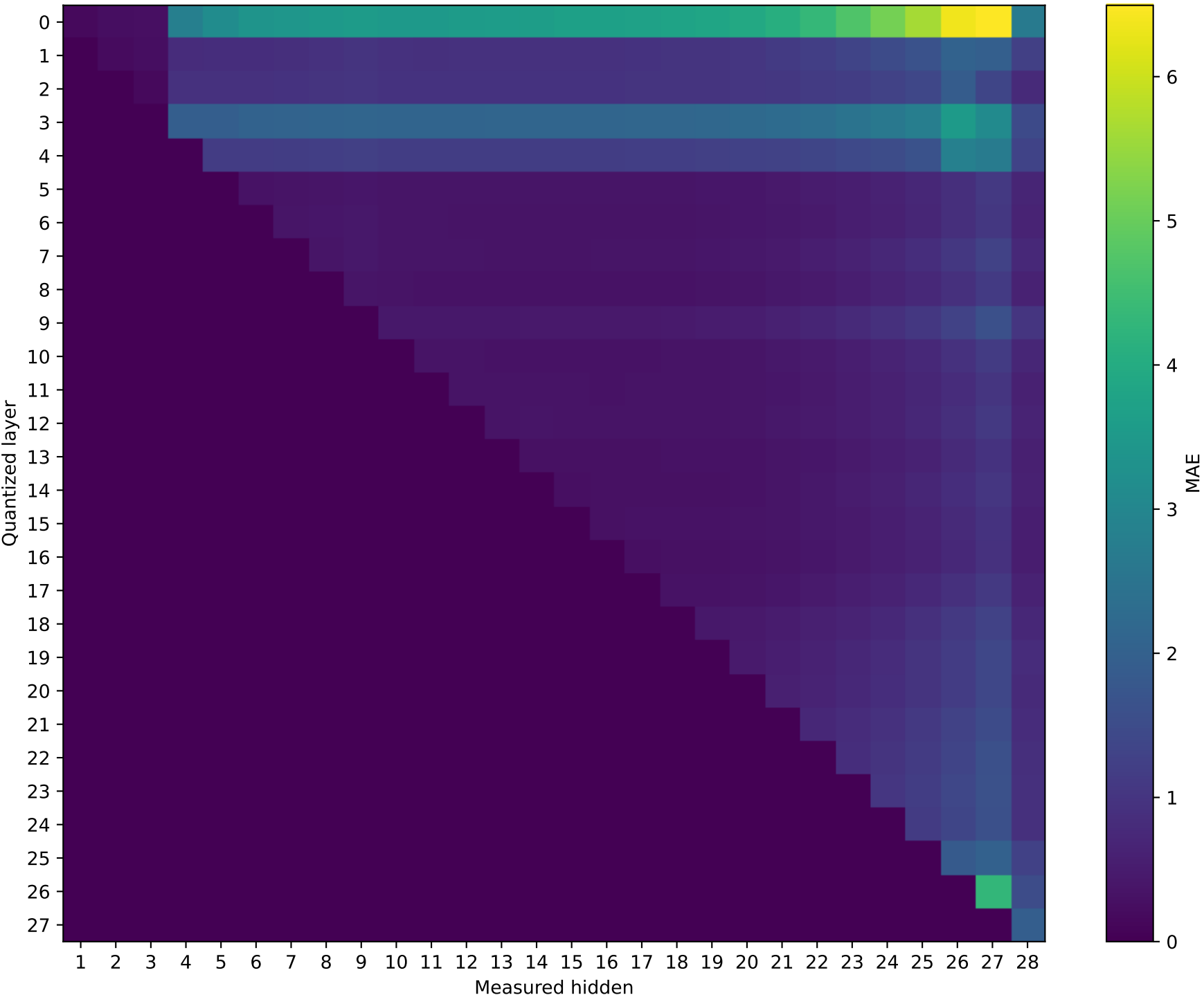
Model: Qwen2.5-7B-Instruct | float32 \rightarrow int4
