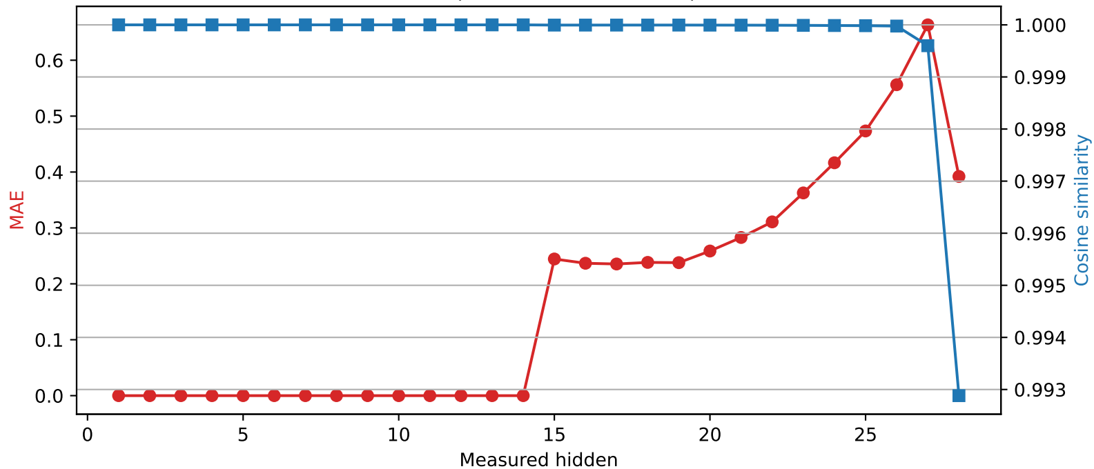
Qwen2.5-7B-Instruct | Quantized layer 14 | float32 \rightarrow int4
