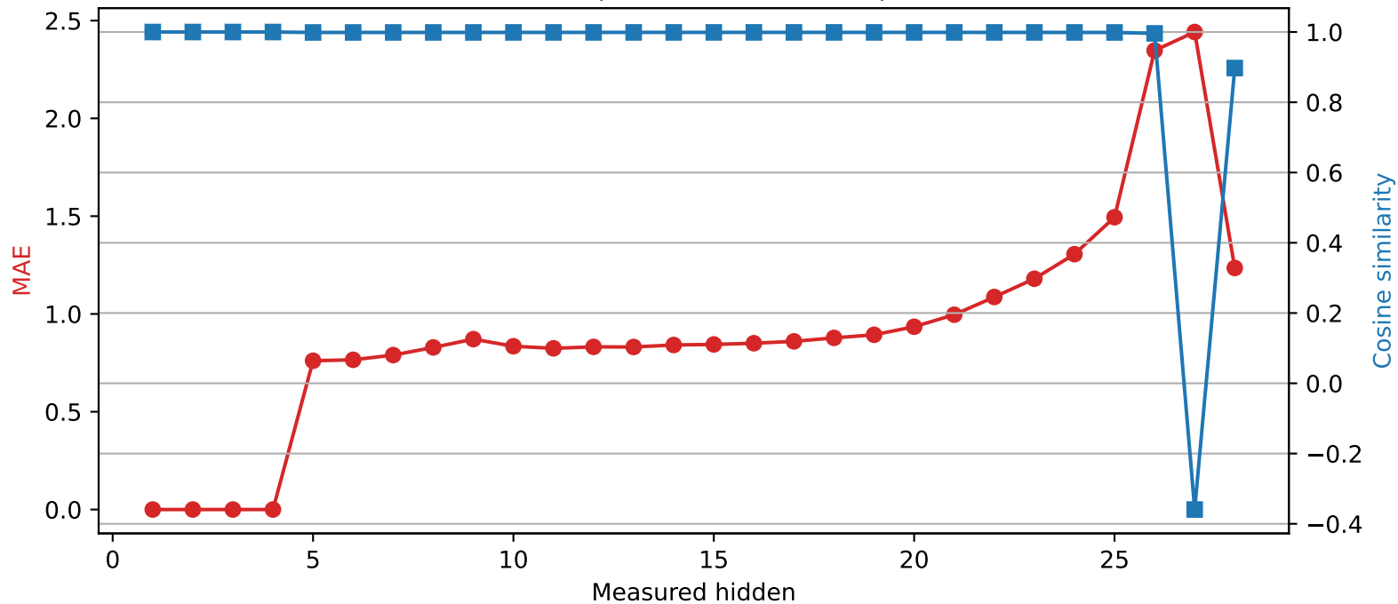
Qwen2.5-7B-Instruct | Quantized layer 4 | float32 \rightarrow int4
