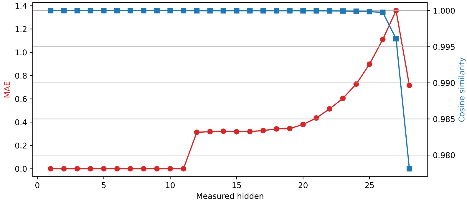
Qwen2.5-7B-Instruct | Quantized layer 11 | float32 \rightarrow int4
