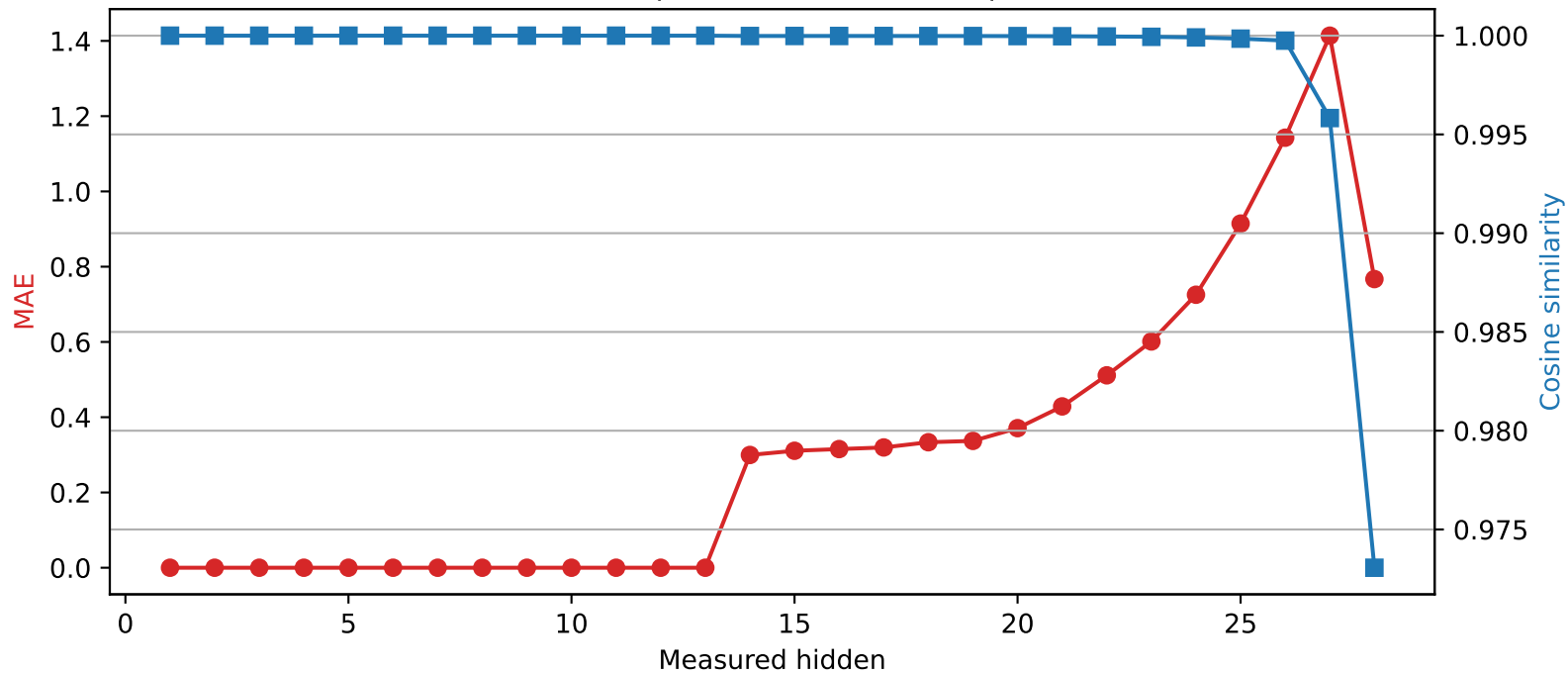
Qwen2.5-7B-Instruct | Quantized layer 13 | float32 \rightarrow int4
