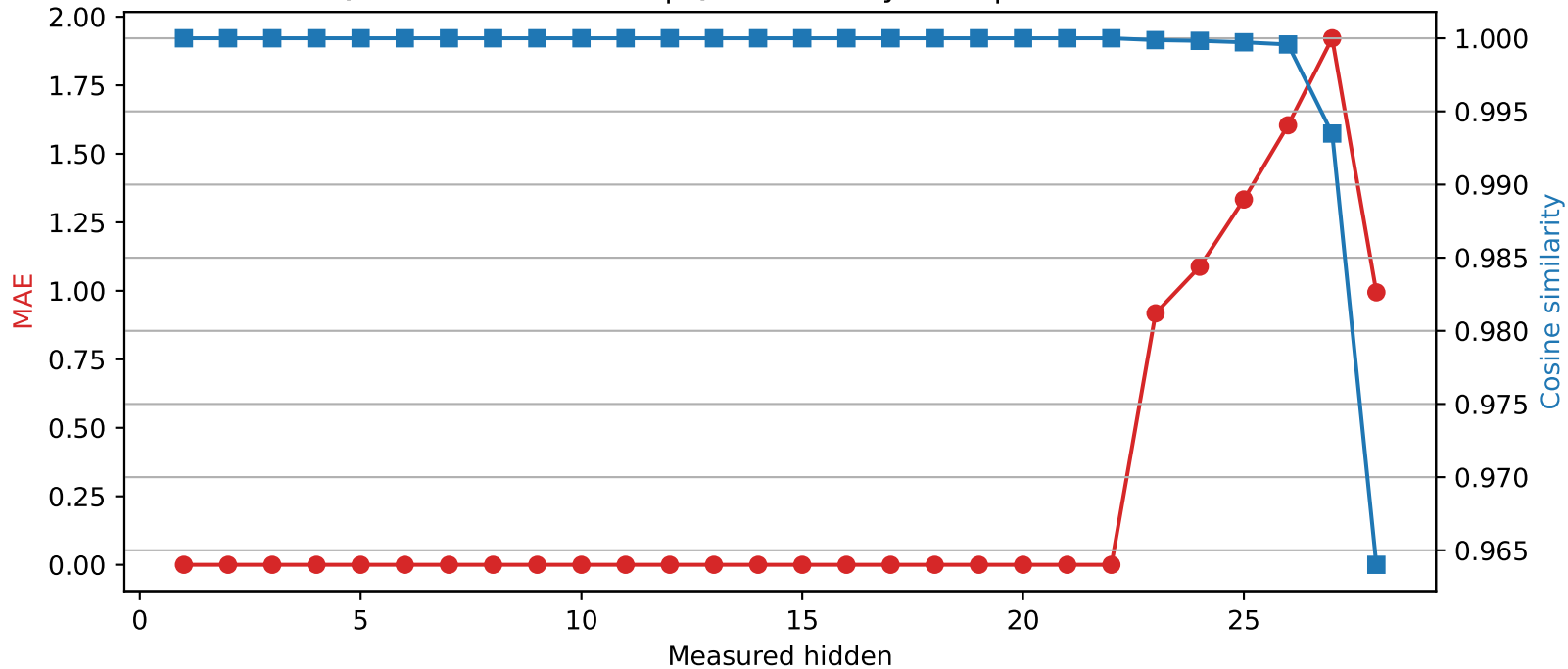
Qwen2.5-7B-Instruct | Quantized layer 22 | float32 → int4
