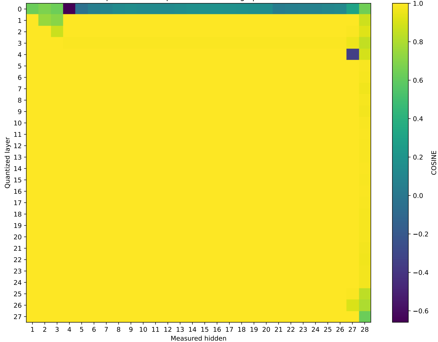
Qwen2.5-7B-Instruct Prompt 2: cos sim representation damage | float32 → int4
