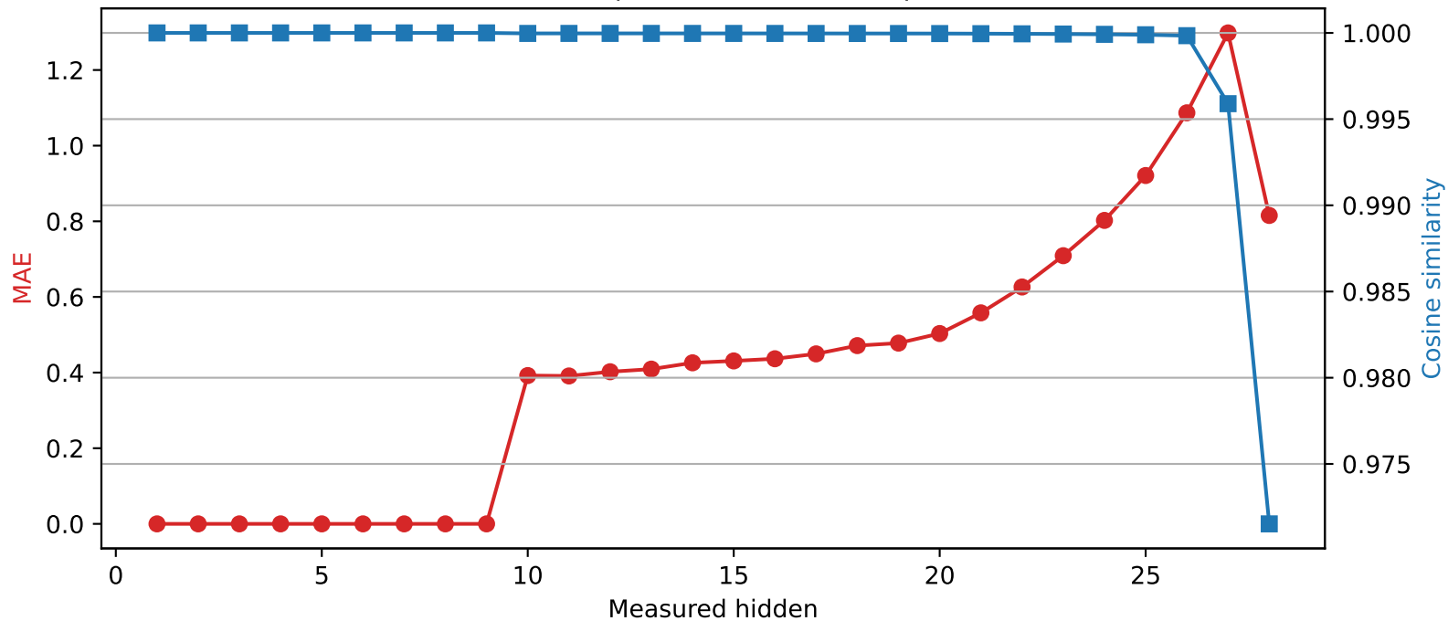
Qwen2.5-7B-Instruct | Quantized layer 9 | float32 \rightarrow int4
