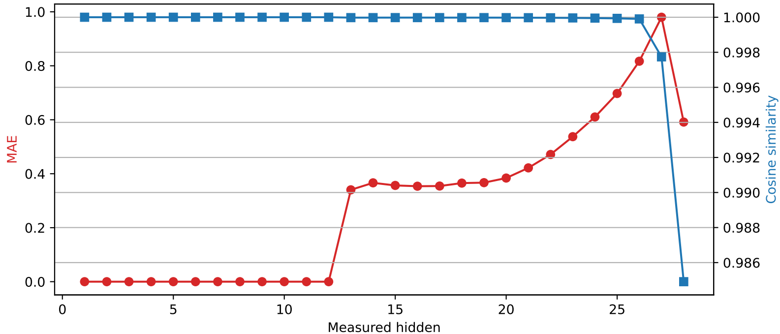
Qwen2.5-7B-Instruct | Quantized layer 12 | float32 → int4
