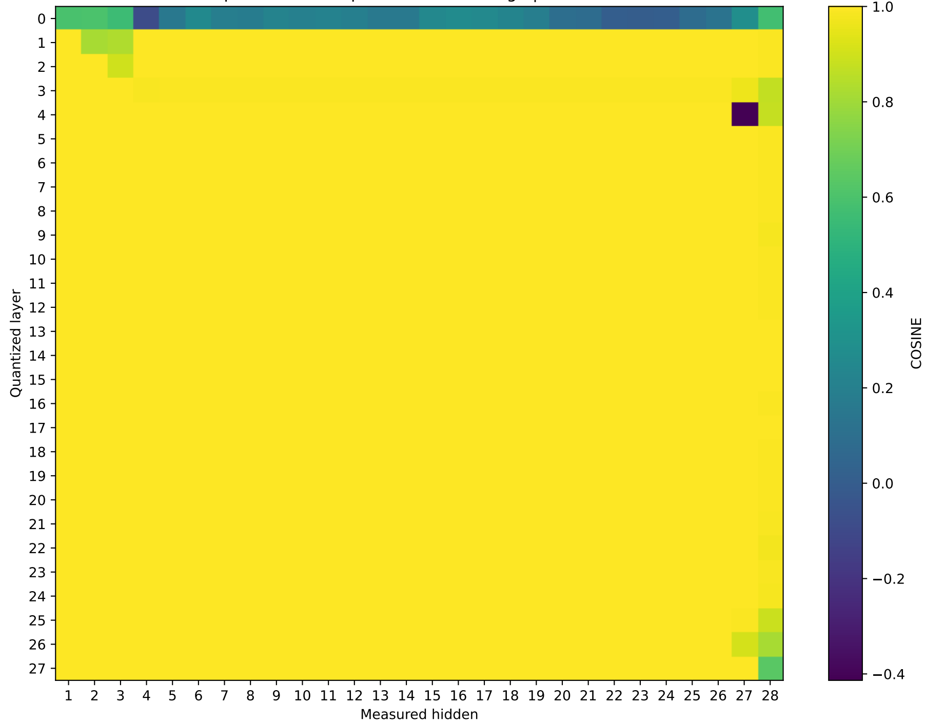
Qwen2.5-7B-Instruct Prompt 4: cos sim representation damage | float32 → int4
