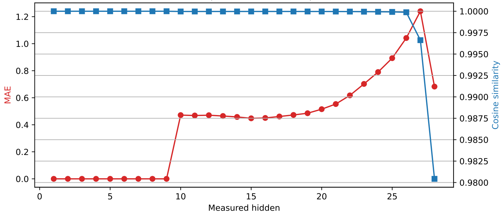
Qwen2.5-7B-Instruct | Quantized layer 9 | float32 → int4
