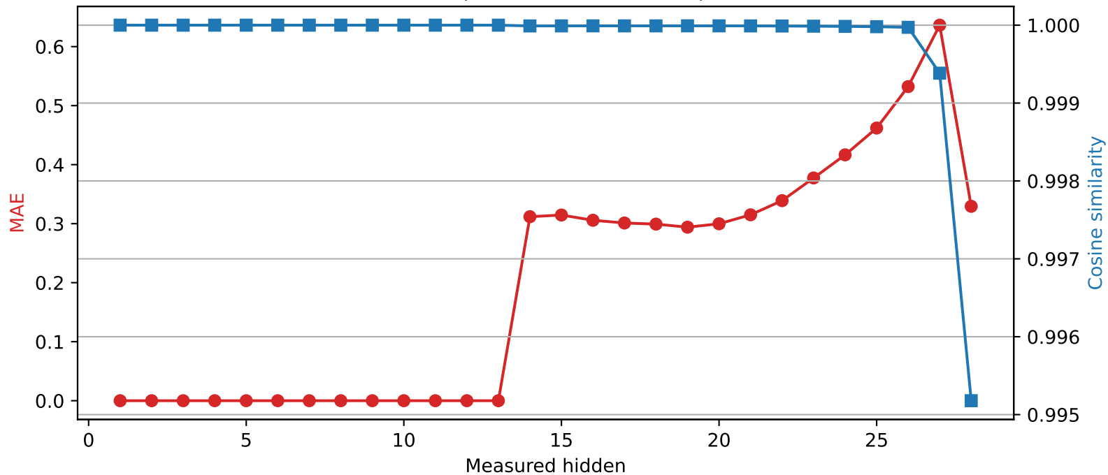
Qwen2.5-7B-Instruct | Quantized layer 13 | float32 → int4
