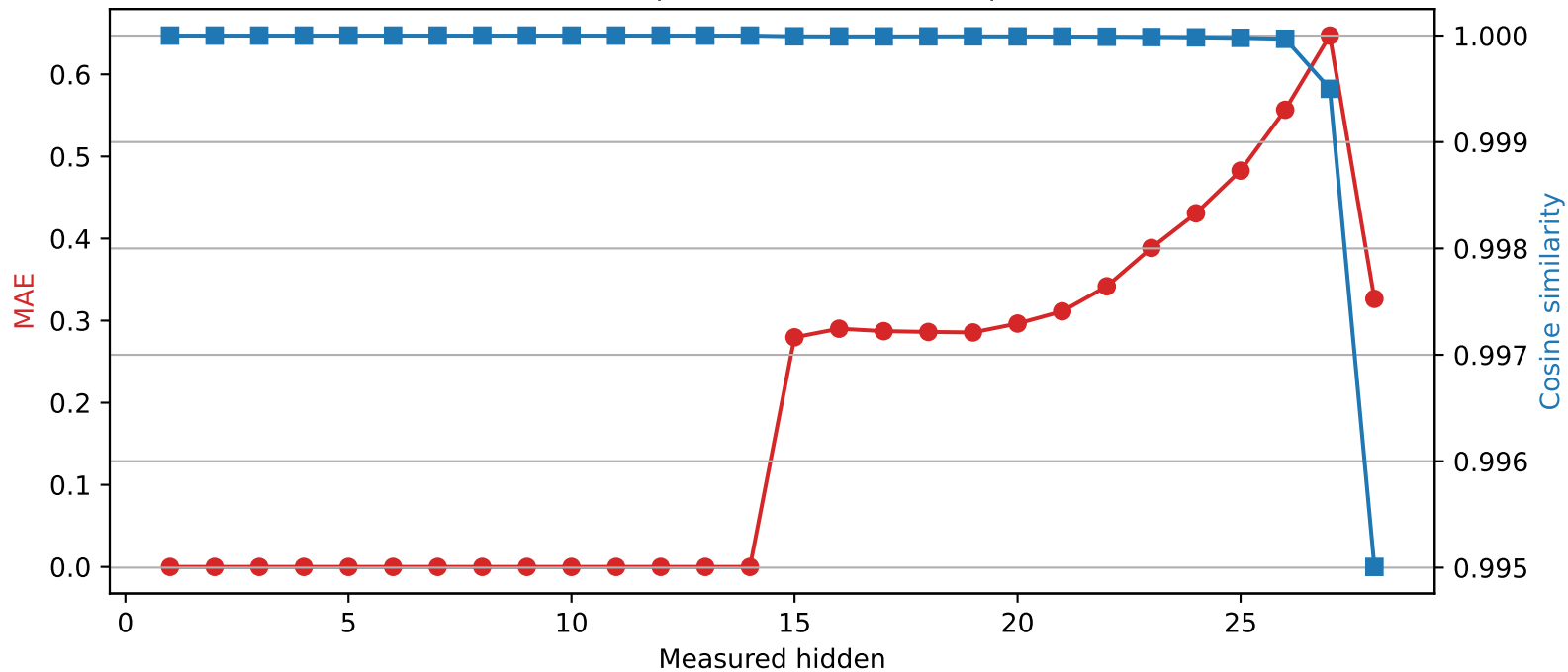
Qwen2.5-7B-Instruct | Quantized layer 14 | float32 → int4
