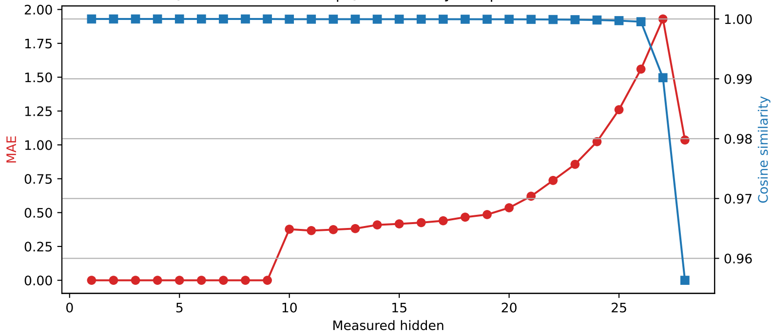
Qwen2.5-7B-Instruct | Quantized layer 9 | float64 → int4
