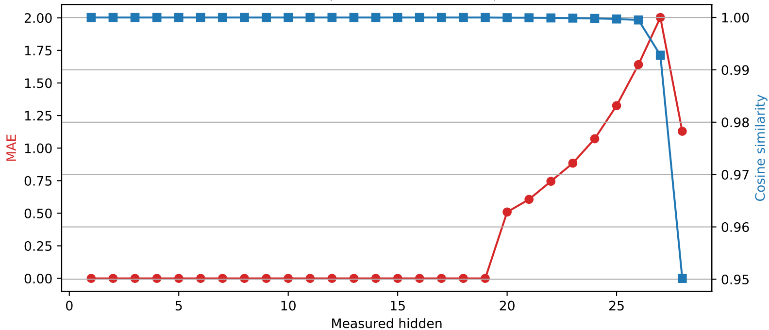
Qwen2.5-7B-Instruct | Quantized layer 19 | float64 \rightarrow int4
