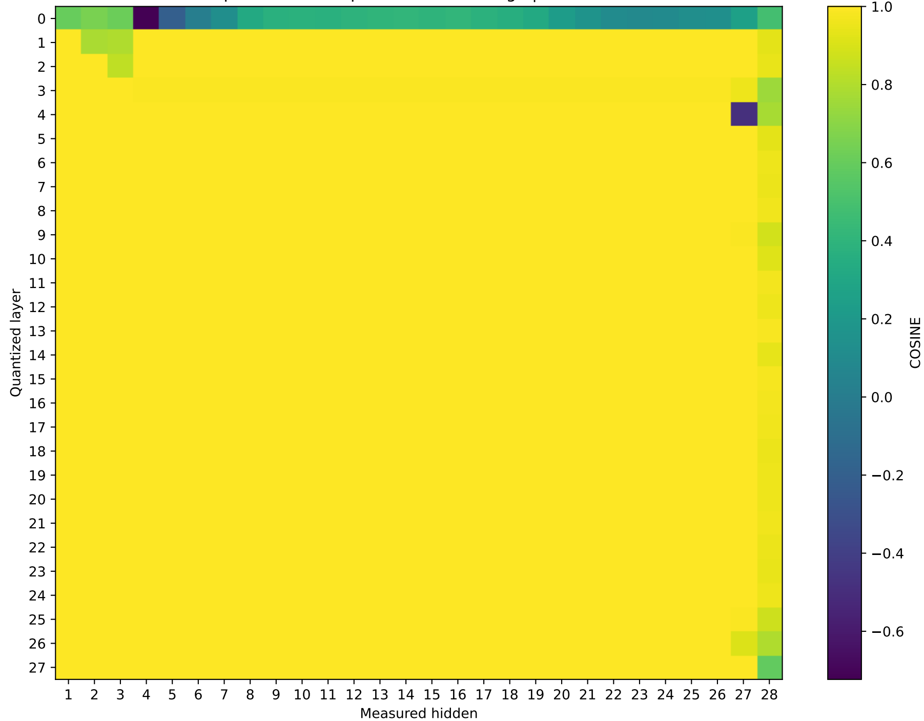
Qwen2.5-7B-Instruct Prompt 3: cos sim representation damage | float64 → int4
