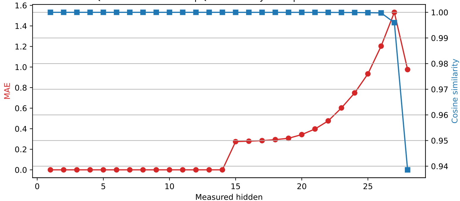
Qwen2.5-7B-Instruct | Quantized layer 14 | float64 \rightarrow int4
