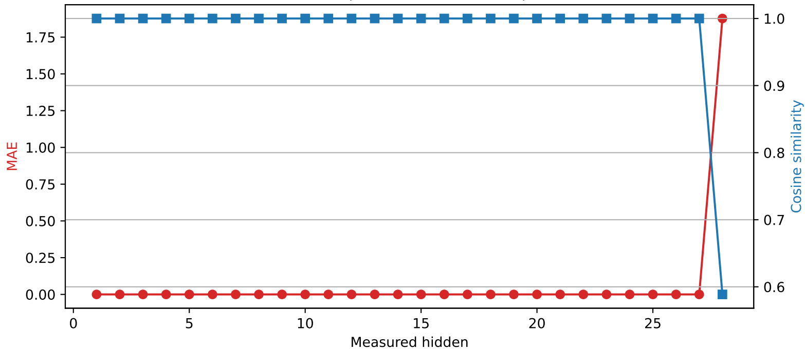
Qwen2.5-7B-Instruct | Quantized layer 27 | float64 → int4
