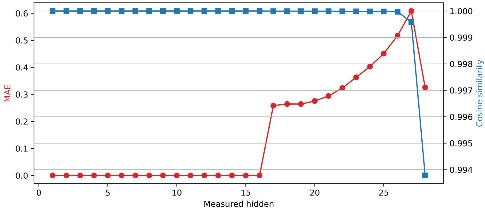
Qwen2.5-7B-Instruct | Quantized layer 16 | float64 → int4
