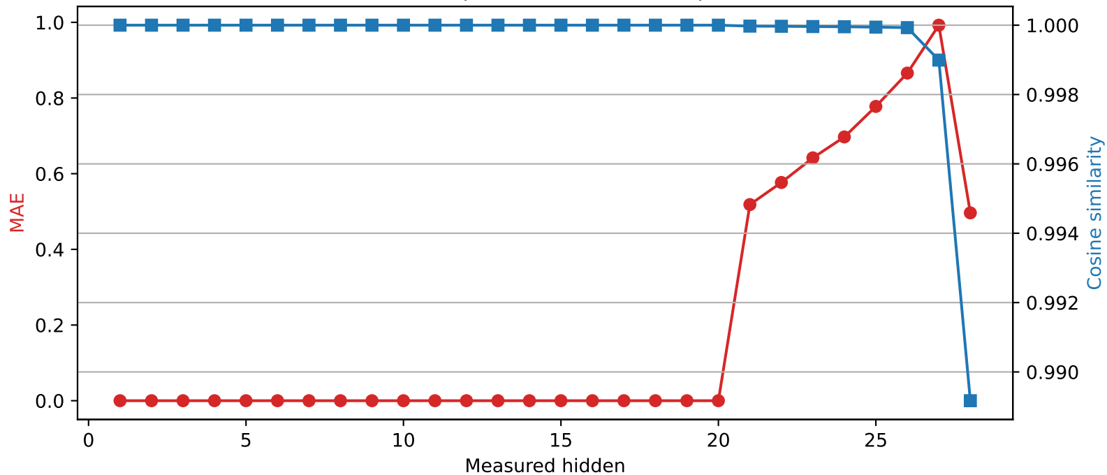
Qwen2.5-7B-Instruct | Quantized layer 20 | float64 → int4
