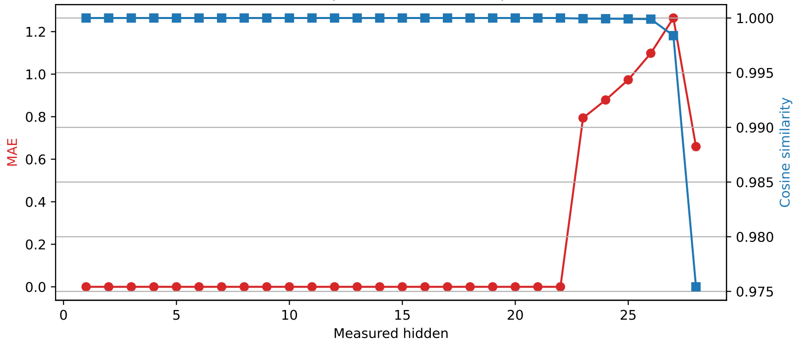
Qwen2.5-7B-Instruct | Quantized layer 22 | float64 → int4
