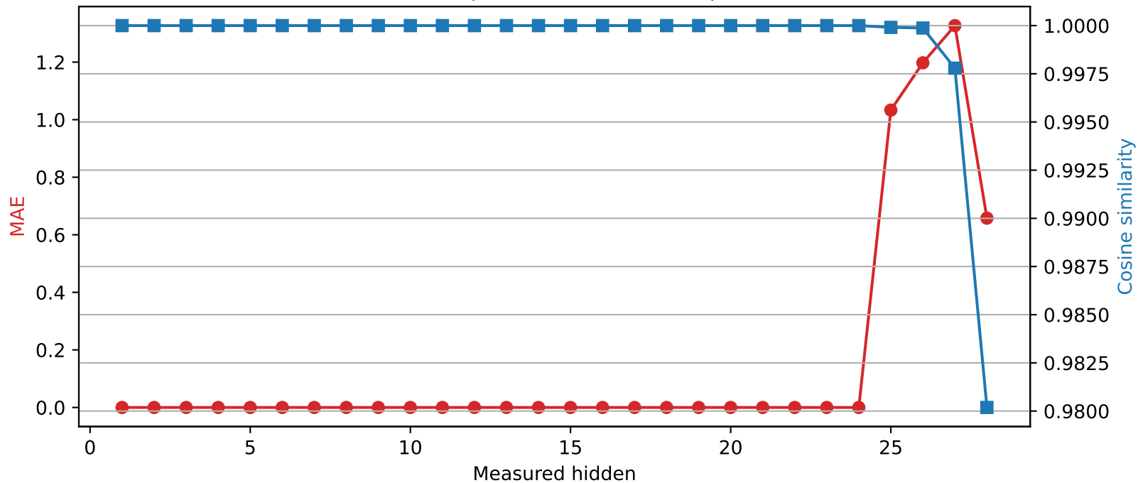
Qwen2.5-7B-Instruct | Quantized layer 24 | float64 → int4
