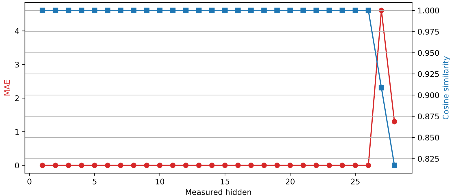
Qwen2.5-7B-Instruct | Quantized layer 26 | float64 → int4
