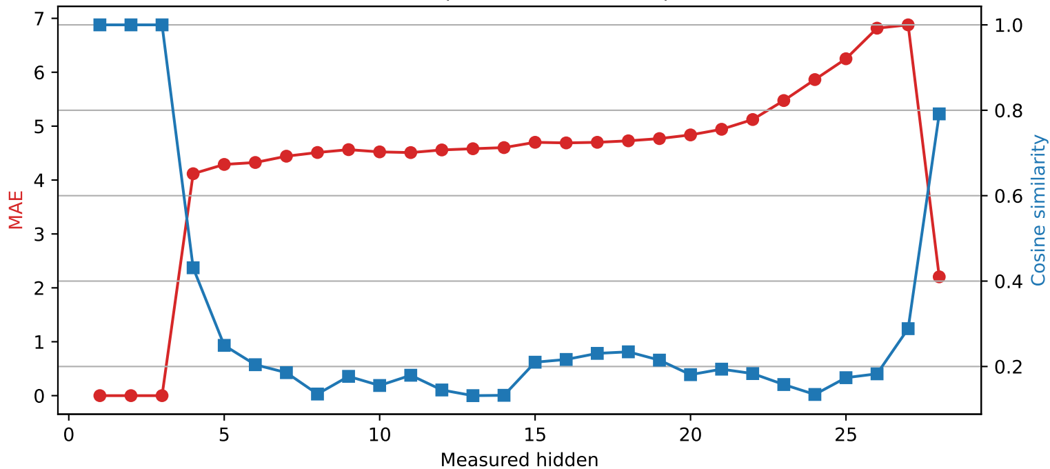
Qwen2.5-7B-Instruct | Quantized layer 3 | float16 → int2
