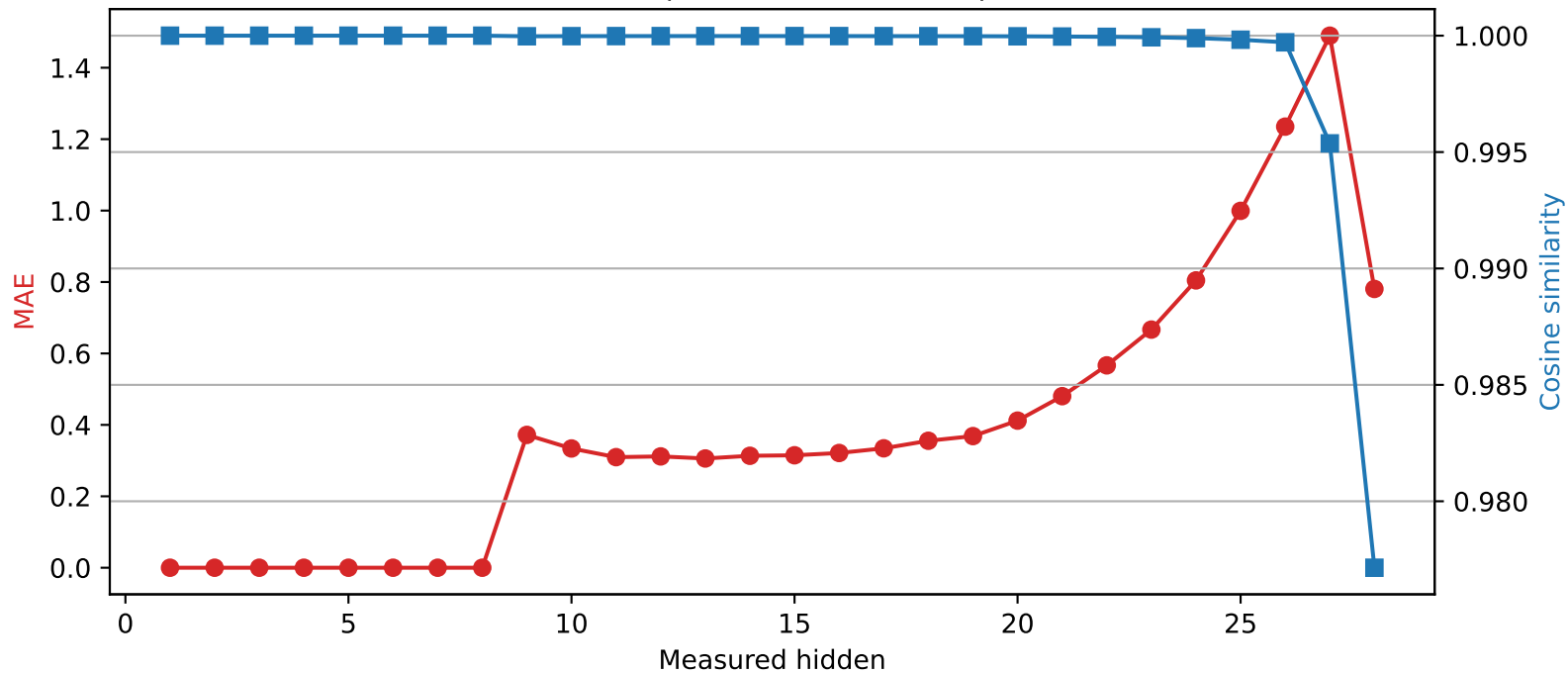
Qwen2.5-7B-Instruct | Quantized layer 8 | float16 \rightarrow int2
