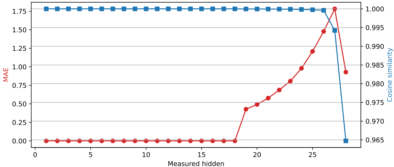
Qwen2.5-7B-Instruct | Quantized layer 18 | float16 → int2
