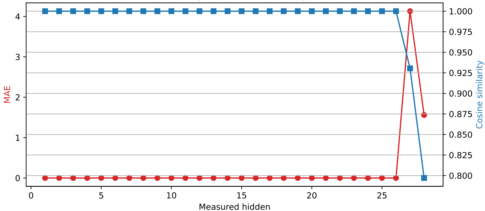
Qwen2.5-7B-Instruct | Quantized layer 26 | float16 → int2
