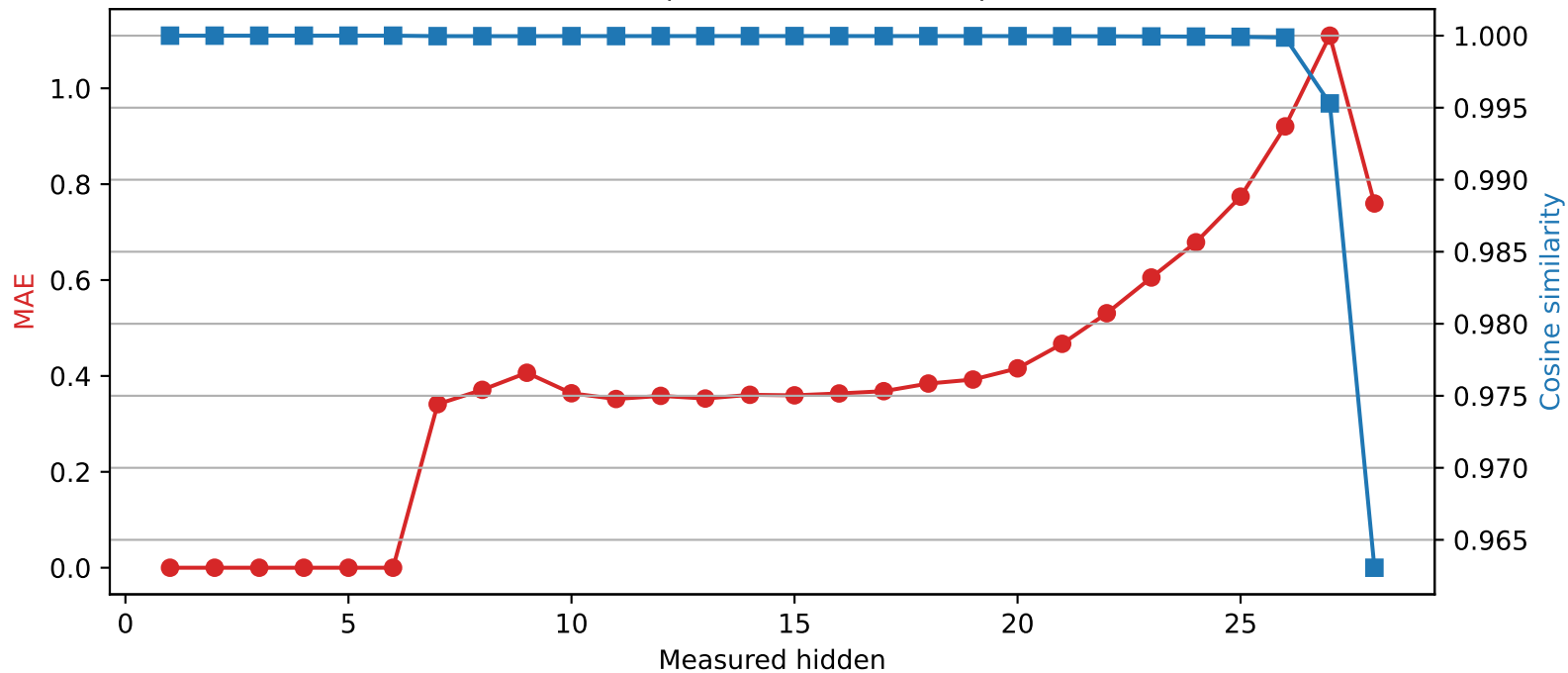
Qwen2.5-7B-Instruct | Quantized layer 6 | float16 → int2
