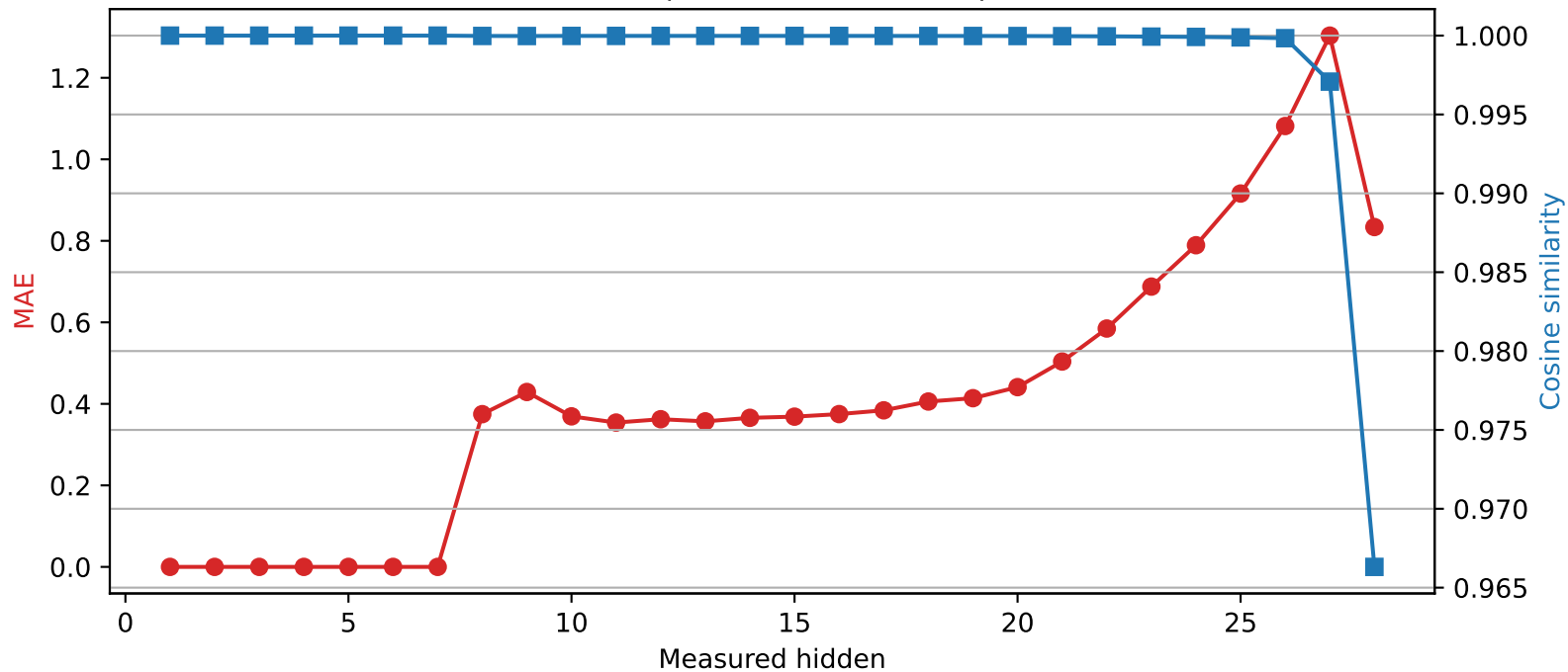
Qwen2.5-7B-Instruct | Quantized layer 7 | float16 → int2
