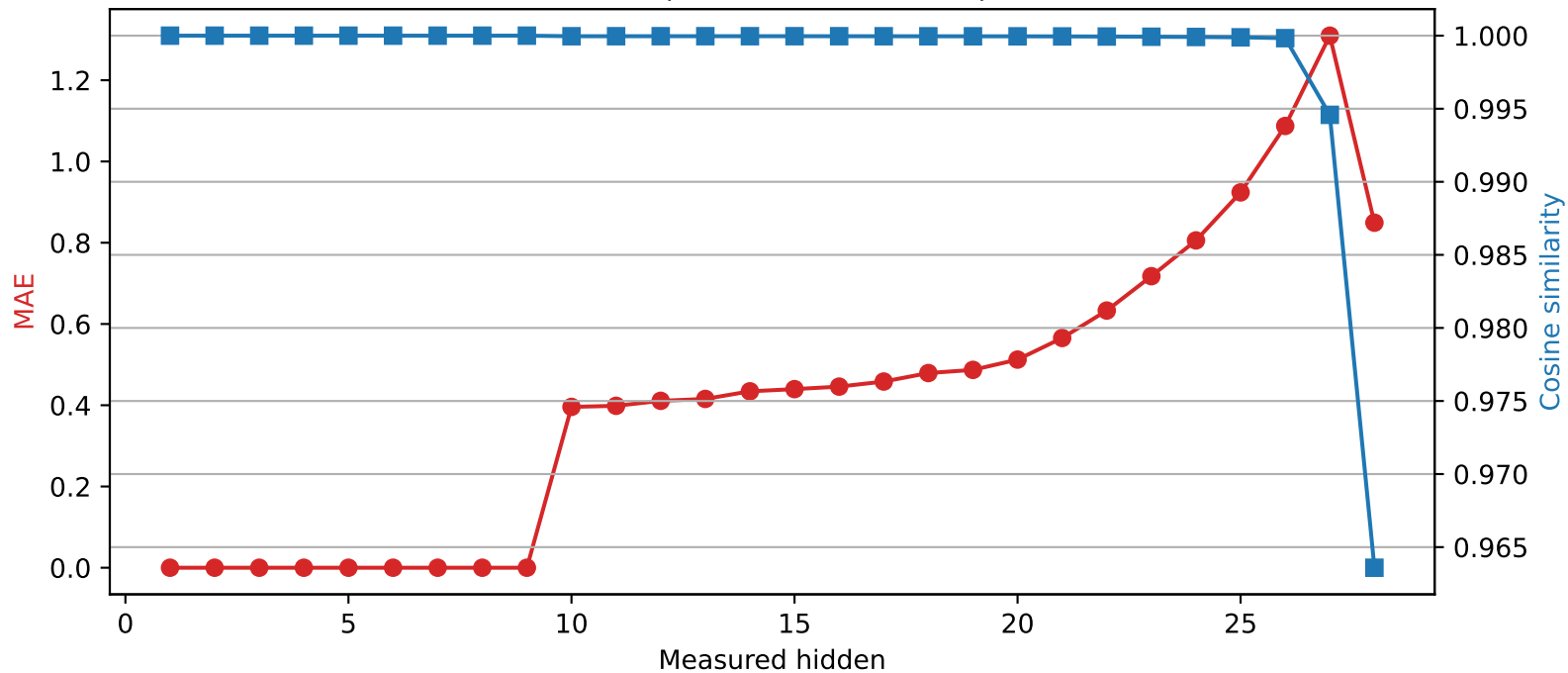
Qwen2.5-7B-Instruct | Quantized layer 9 | float16 → int2
