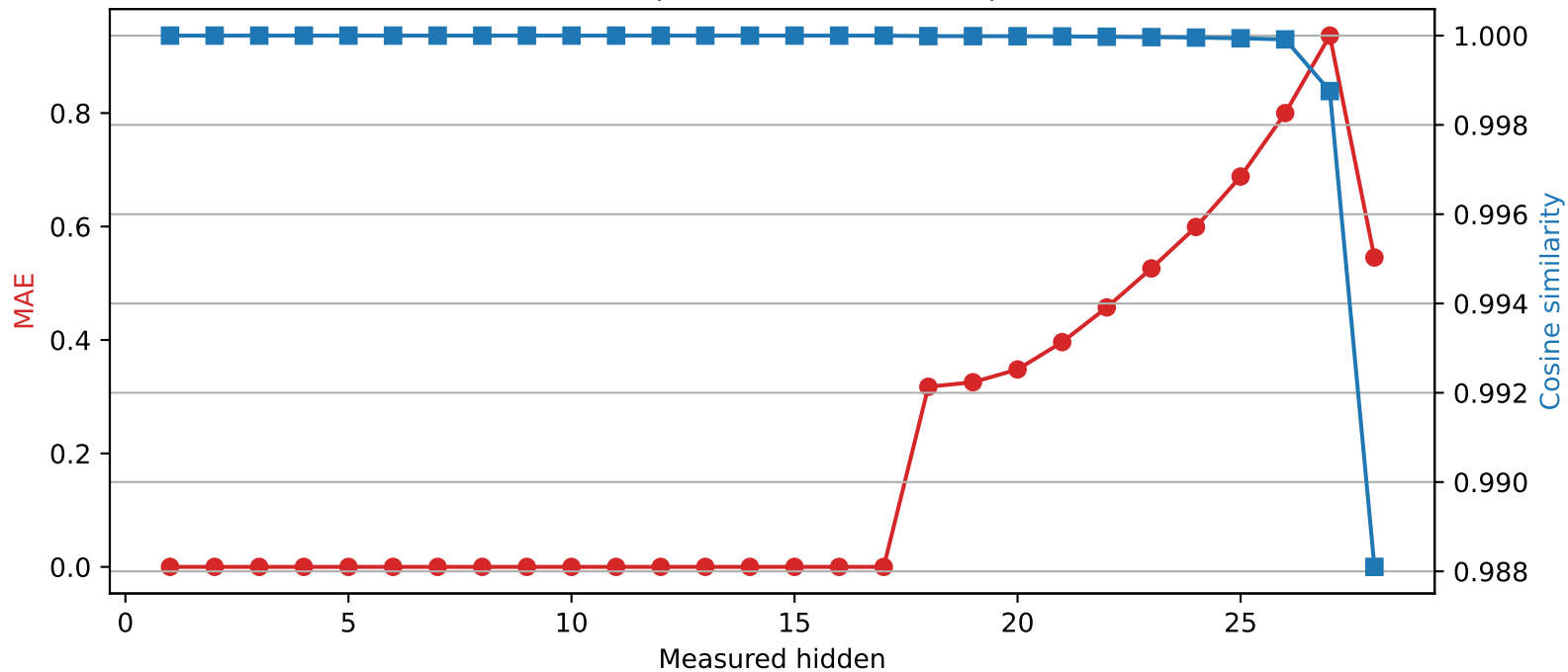
Qwen2.5-7B-Instruct | Quantized layer 17 | float16 → int2
