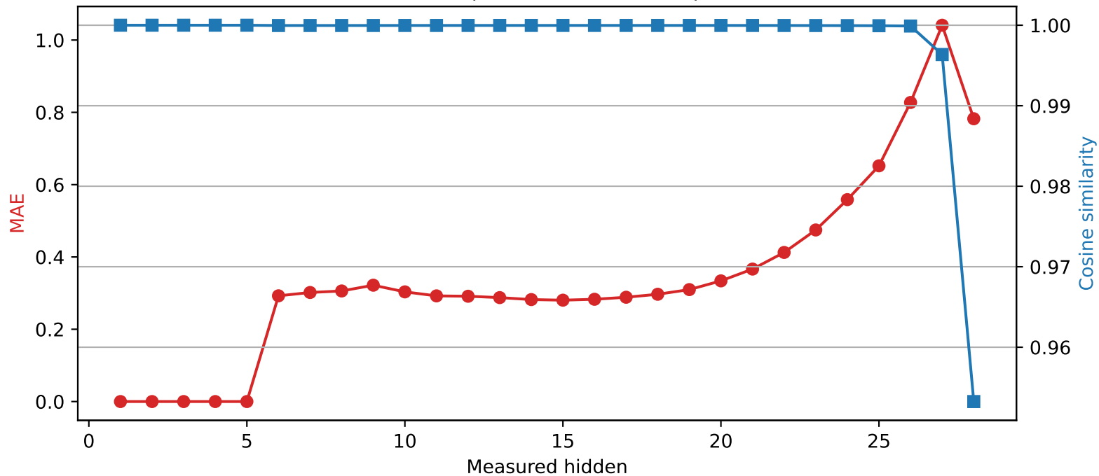
Qwen2.5-7B-Instruct | Quantized layer 5 | float16 → int2
