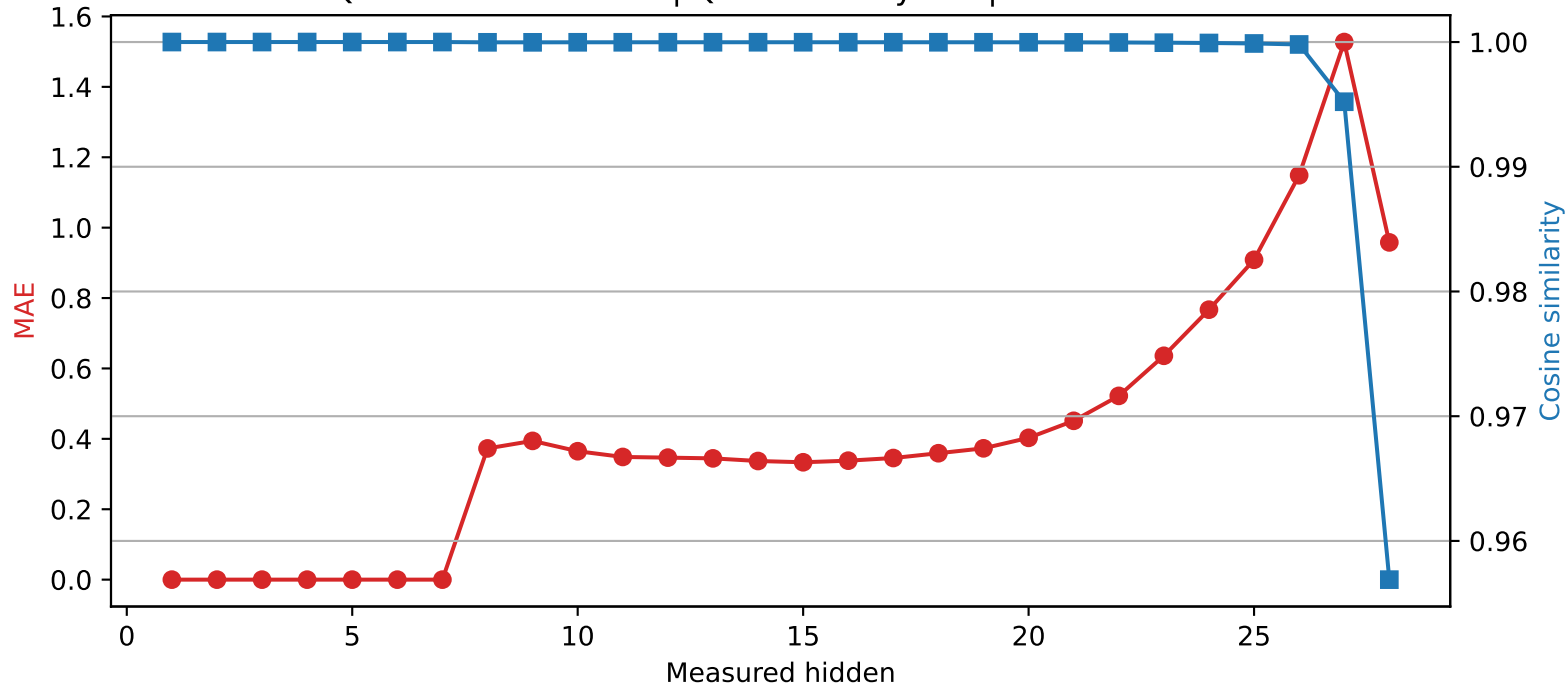
Qwen2.5-7B-Instruct | Quantized layer 7 | float16 \rightarrow int2
