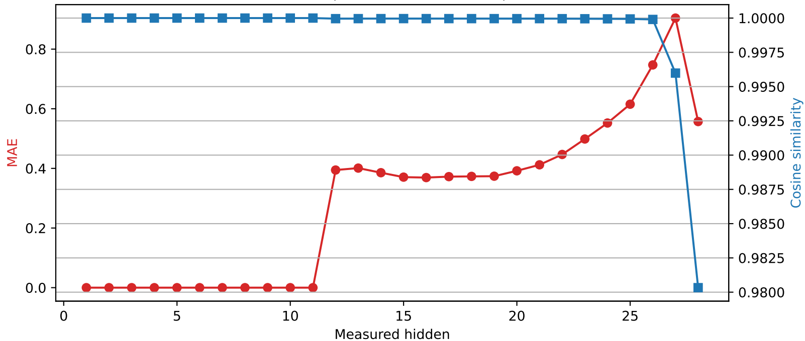
Qwen2.5-7B-Instruct | Quantized layer 11 | float16 → int2
