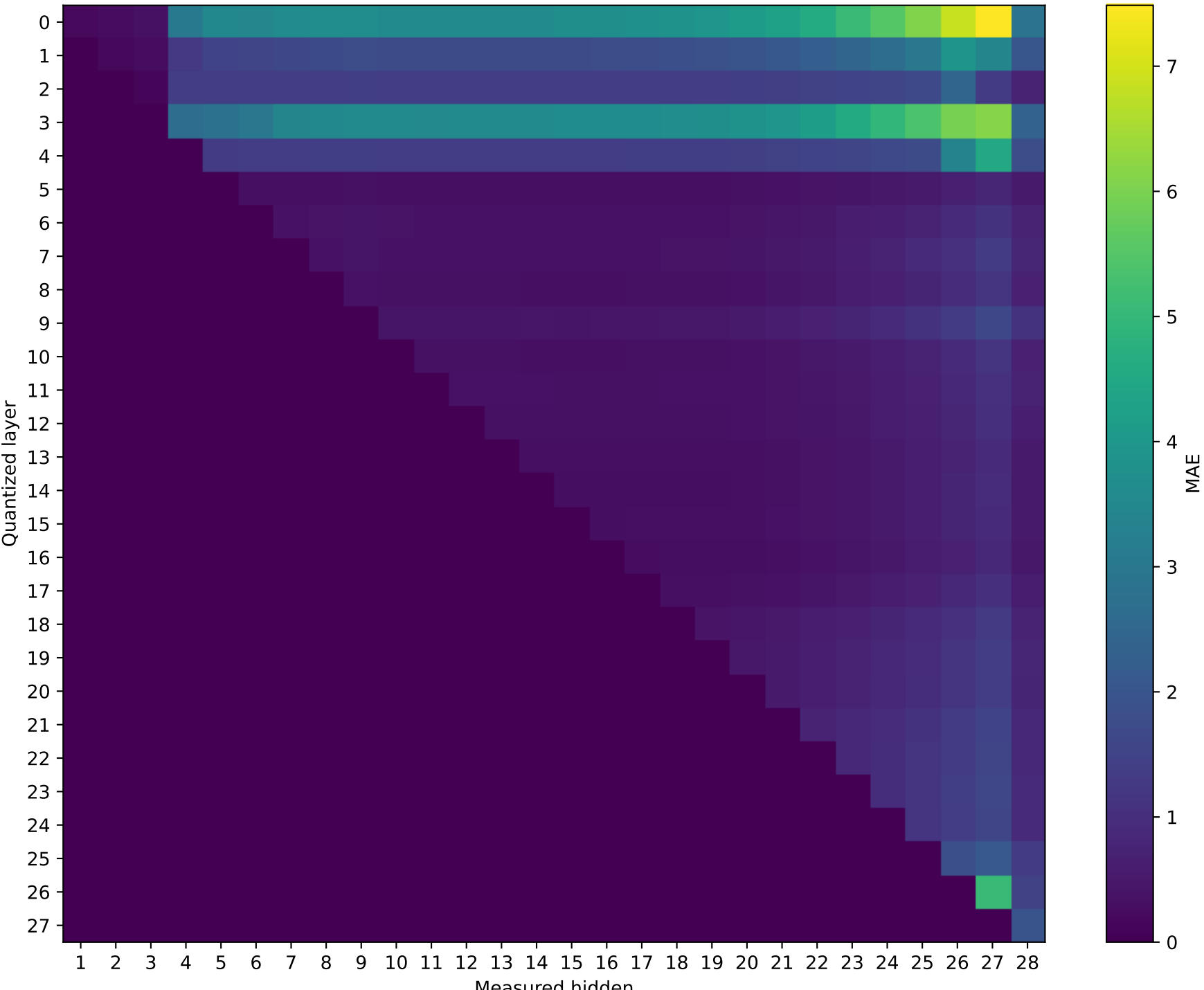
Model: Qwen2.5-7B-Instruct | float32 → int2
