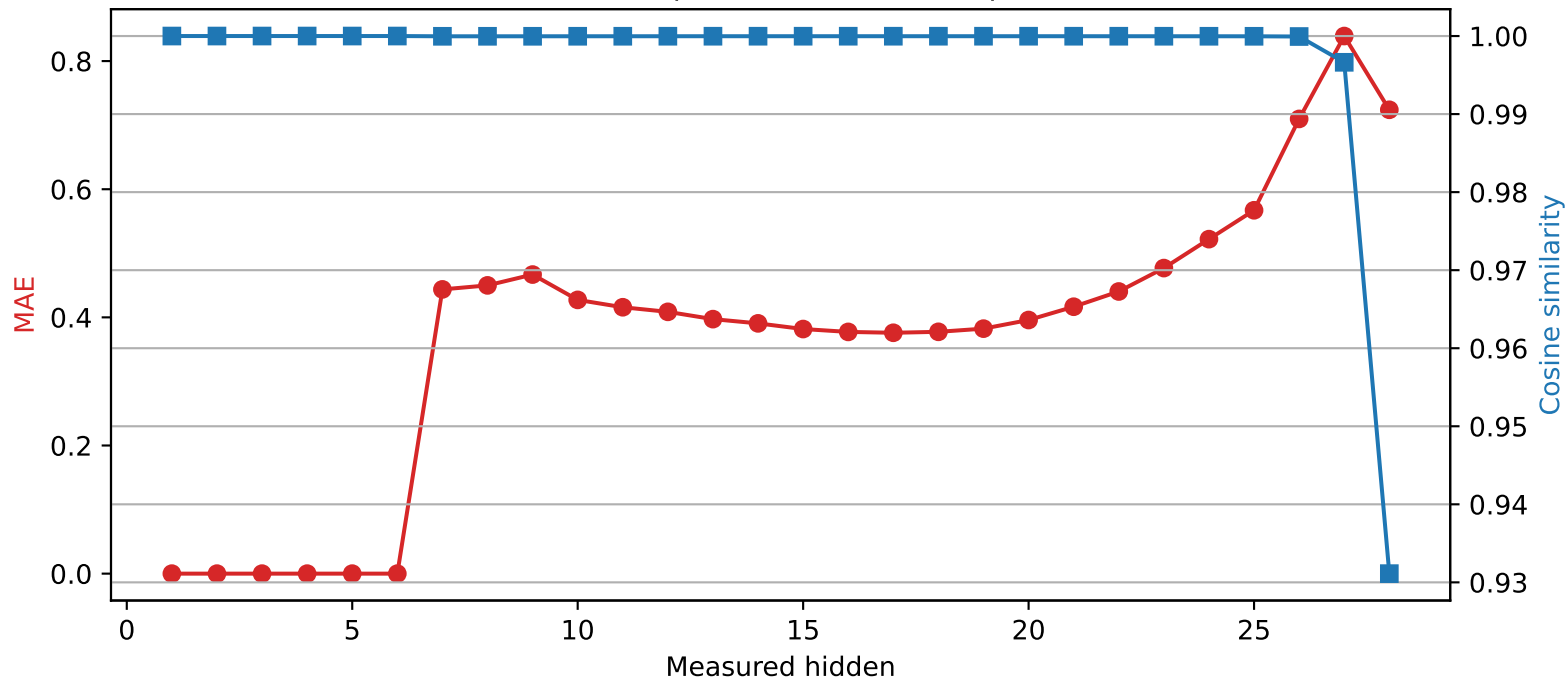
Qwen2.5-7B-Instruct | Quantized layer 6 | float32 → int2
