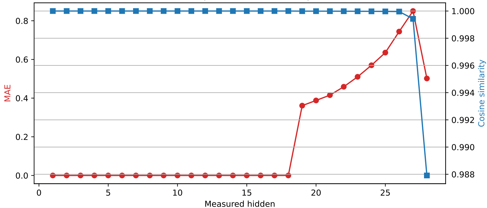
Qwen2.5-7B-Instruct | Quantized layer 18 | float32 → int2
