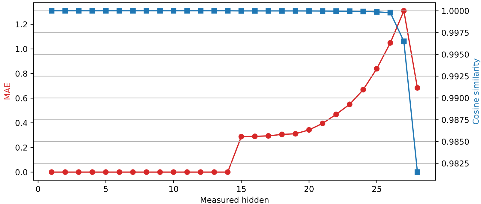
Qwen2.5-7B-Instruct | Quantized layer 14 | float32 → int2
