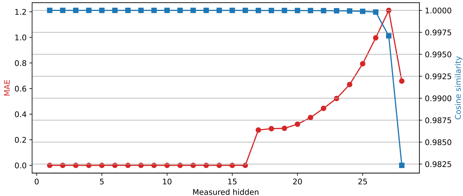
Qwen2.5-7B-Instruct | Quantized layer 16 | float32 → int2
