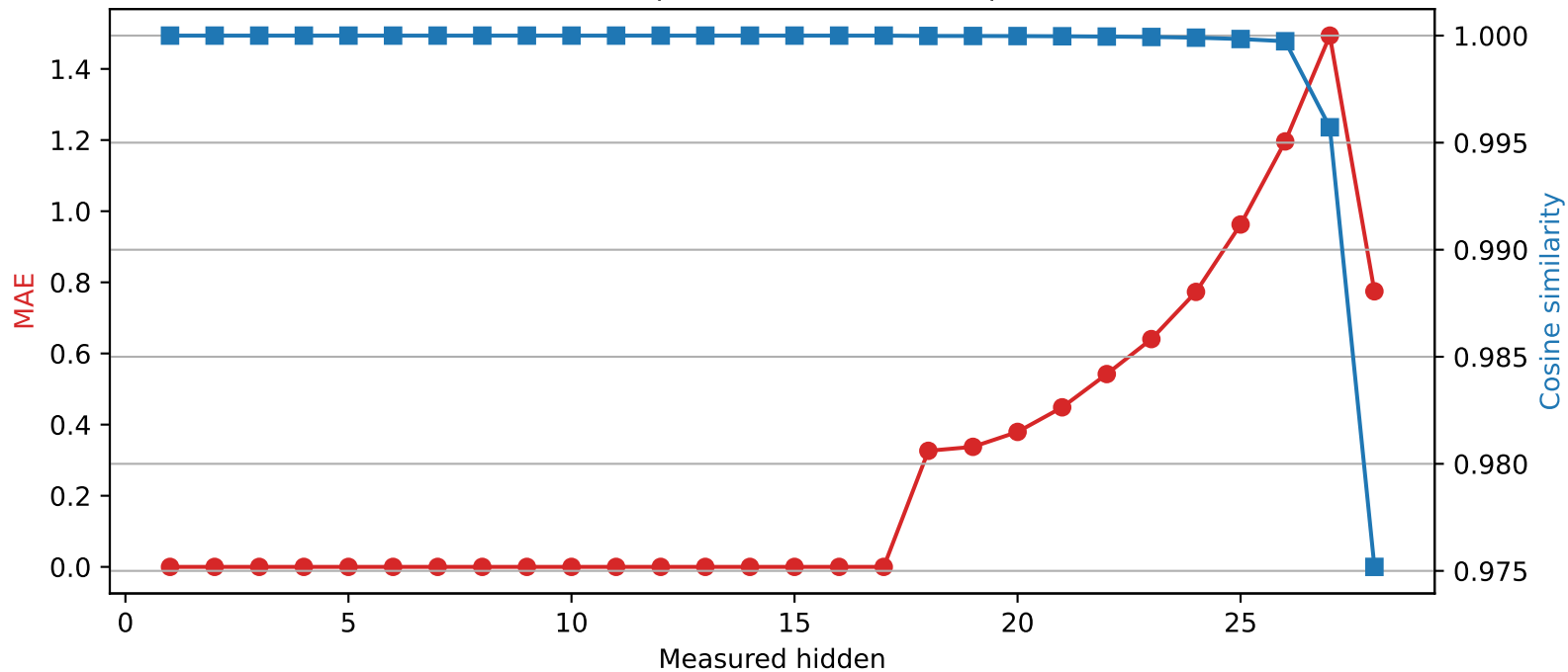
Qwen2.5-7B-Instruct | Quantized layer 17 | float32 \rightarrow int2
