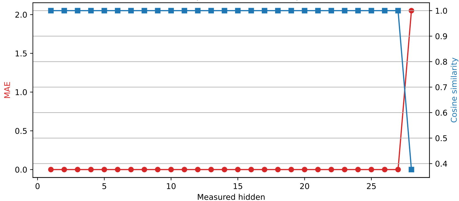
Qwen2.5-7B-Instruct | Quantized layer 27 | float32 \rightarrow int2
