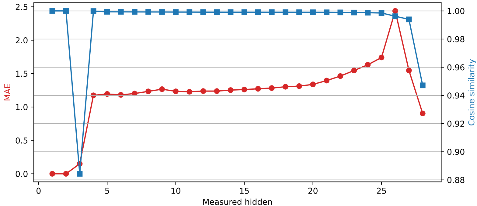
Qwen2.5-7B-Instruct | Quantized layer 2 | float32 \rightarrow int2
