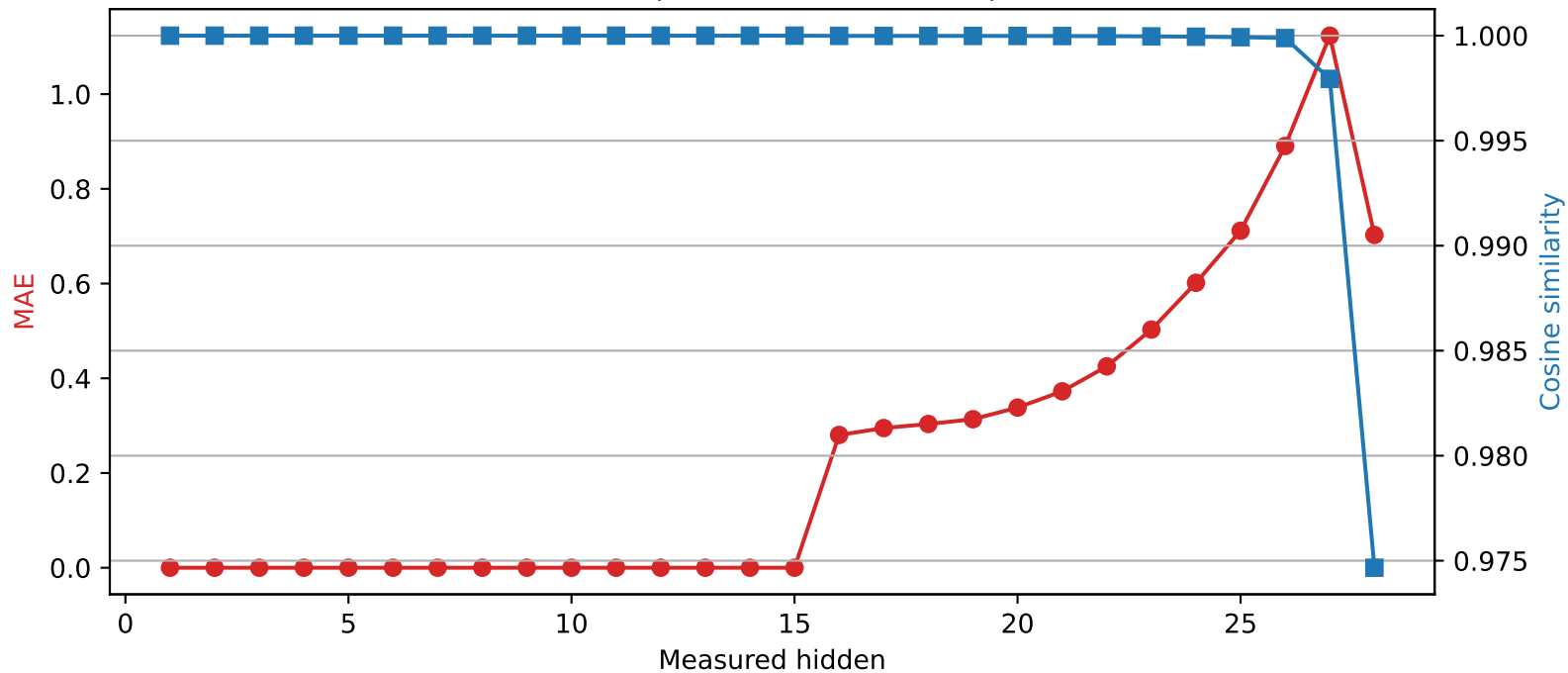
Qwen2.5-7B-Instruct | Quantized layer 15 | float32 → int2
