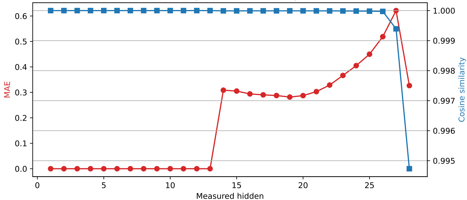
Qwen2.5-7B-Instruct | Quantized layer 13 | float32 → int2
