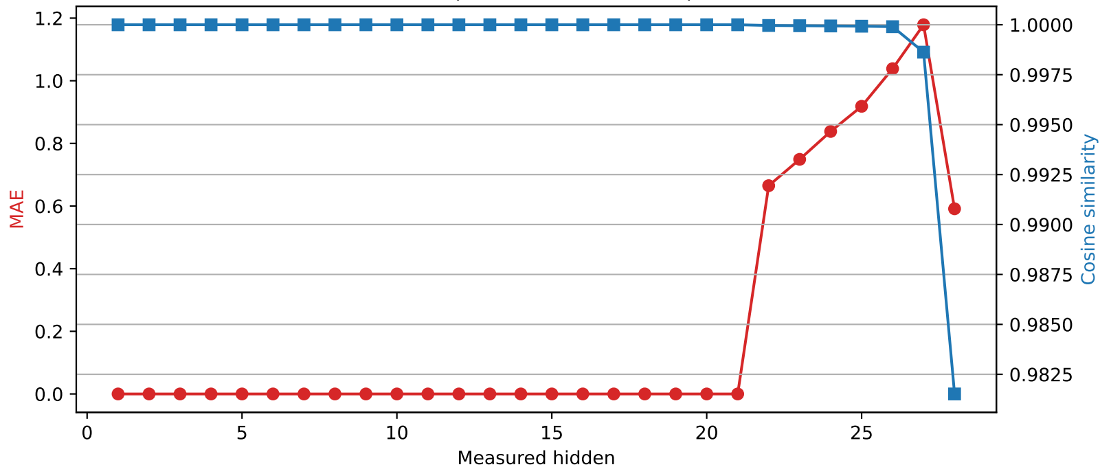
Qwen2.5-7B-Instruct | Quantized layer 21 | float32 → int2
