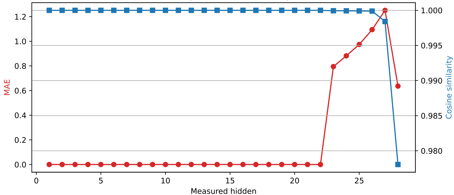
Qwen2.5-7B-Instruct | Quantized layer 22 | float32 → int2
